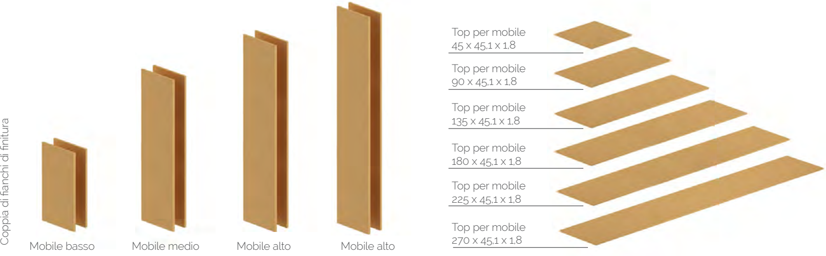
Mobile basso Mobile medio Mobile alto Mobile alto 1.8 x 45.1 x 86 h 2.5 x 45.1 x 86.7 h 3.8 x 45.1 x 88 h 1.8 x 45.1 x 166 h 2.5 x 45.1 x 166.7 h 3.8 x 45.1 x 168 h 1.8 x 45.1 x 206 h 2.5 x 45.1 x 206.7 h 3.8 x 45.1 x 208 h 1.8 x 45.1 x 246 h 2.5 x 45.1 x 246.7 h 3.8 x 45.1 x 248 h
